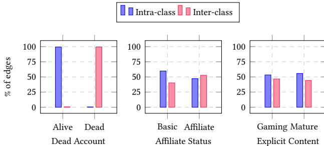
Figure 1: The percentage of intra and inter-class edges conditional on the Dead Account , Affiliate Status , and Explicit Content attributes.
