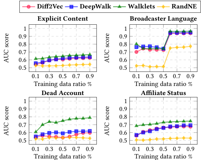
Figure 5: Predictive performance of proximity preserving node embedding techniques on classification tasks measured by area under the curve scores on the test set as a function of training set ratio.
