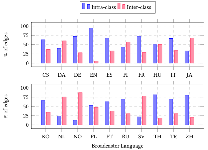
Figure 2: The percentage of intra and inter-class edges conditional on the Broadcaster Language attribute.
